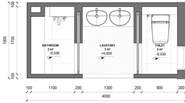
FLOOR PLAN
