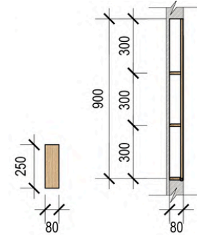
SECTION WALL CABINET
