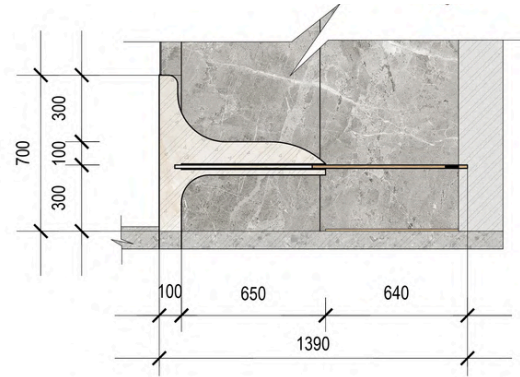
SECTION WALL SEAT
