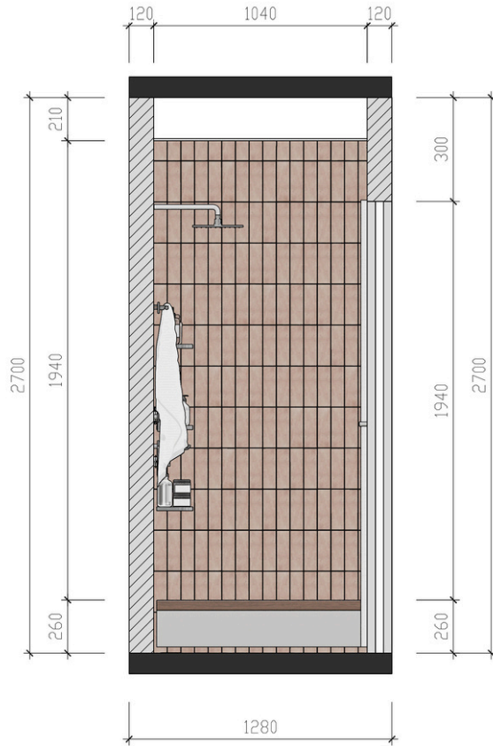
SECTION 03
