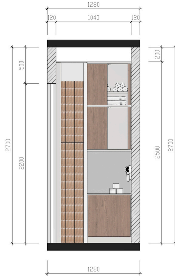
SECTION 04
