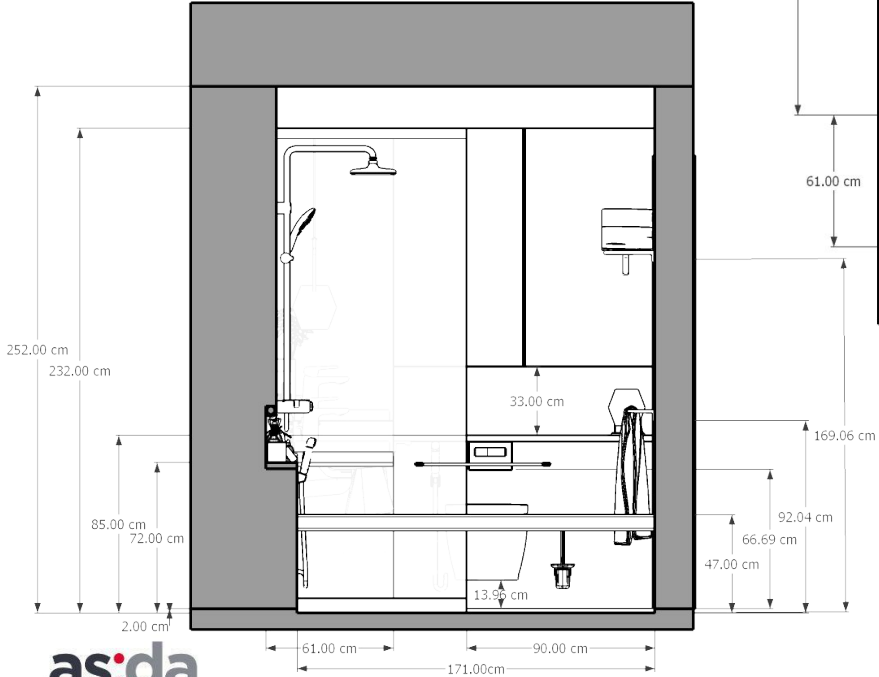
Left Elevation
