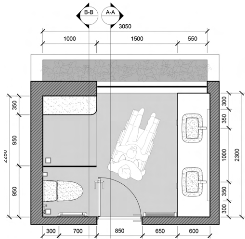
FLOOR PLAN
