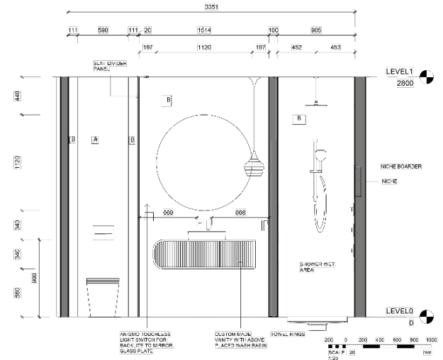
BATHROOM ELEVATION A103
