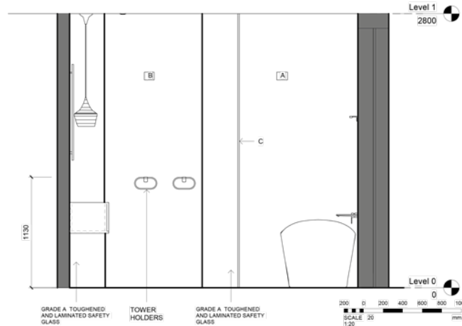
BATHROOM ELEVATION A105
