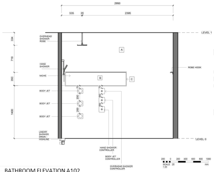
BATHROOM ELEVATION A102
