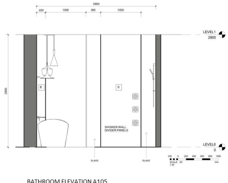
BATHROOM ELEVATION A105
